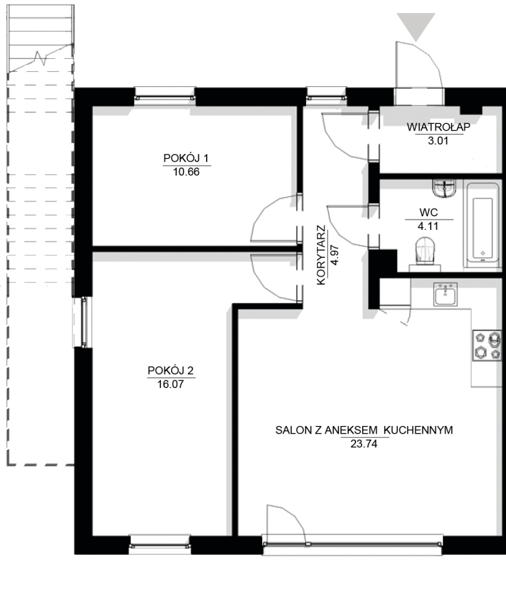
PARTER
